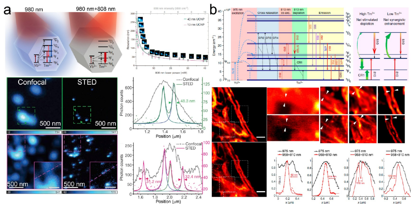
Figure 5. UCNP for super-resolution nanoscopy. (a) Energy diagram of high concentration of \text{Tm}^{3+} doped UCNP with two illumination schemes (left top panel). Relationship of STED resolution of single-particle UCNP and the 808 nm depletion laser intensity (right top panel). Confocal and STED nanoscopy of 8% \text{Tm}^{3+} -doped UCNP and corresponding line-scan profiles (lower panel). Adapted with permission from ref 132, Copyright 2017, Nature Publishing Group. (b) Optical depletion mechanism of the 455 nm upconversion luminescence in \text{NaYF}_4:18\% \text{Yb}^{3+}, 10\% \text{Tm}^{3+} ; STED nanoscopy of UCNP labeled cytoskeleton. Adapted with permission from ref 133, Copyright 2017, Nature Publishing Group.
