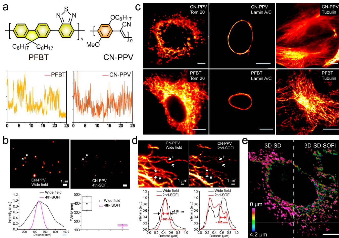
Figure 6. Small photoblinking Pdts for SOFI nanoscopy. (a) Chemical structures and single-particle photoblinking of PFBT and CN-PPV Pdts. (b) Single-particle SOFI nanoscopy of CN-PPV and corresponding spatial resolution. (c) Subcellular specific labeling images of PFBT and CN-PPV Pdts. (d) Wide-field microscopy and SOFI nanoscopy images of CN-PPV labeled microtubules in BS-C-1 cells. (e) Three-dimensional SOFI of CN-PPV Pdts labeled mitochondria membrane in BS-C-1 cell. Scale bar: 1, 10, and 10 \mu\text{m} for (b), (c), and (e), respectively. Adapted with permission from ref 169, Copyright 2017, John Wiley and Sons.
